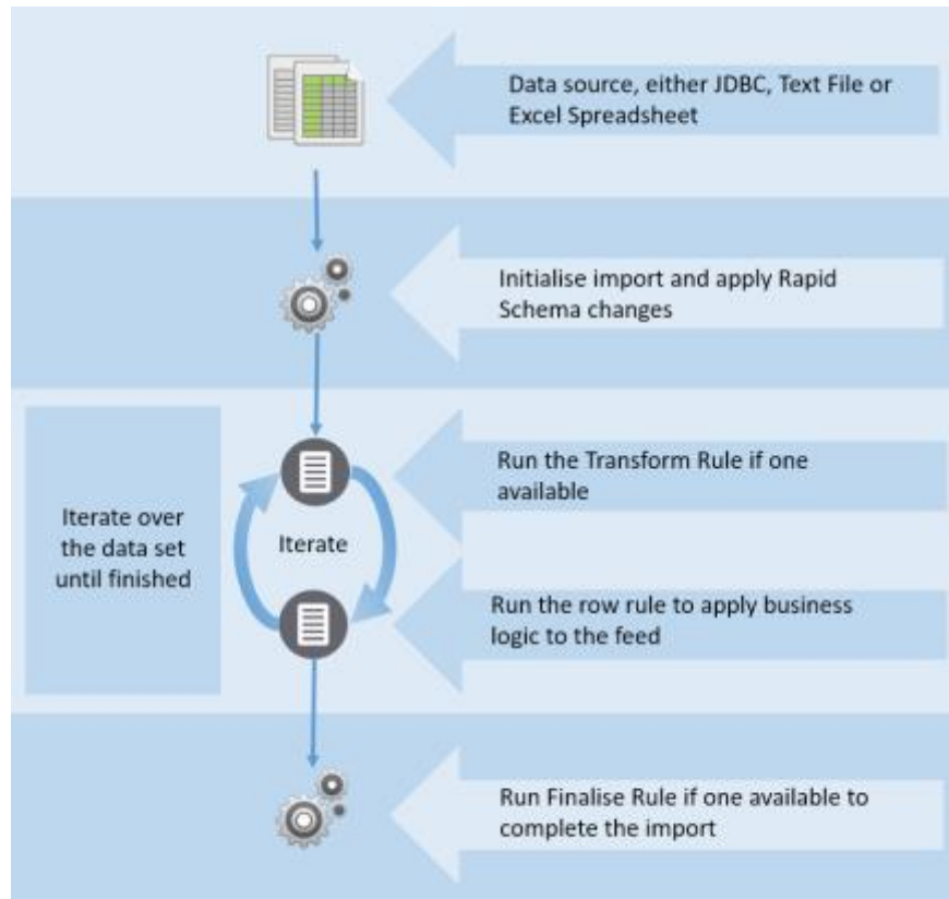
Figure 1: GenericImporter overview
